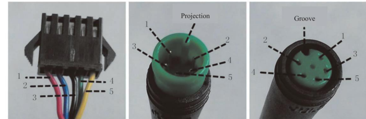
Connecting terminal to the controller Leading-out terminal of display Connecting terminal
